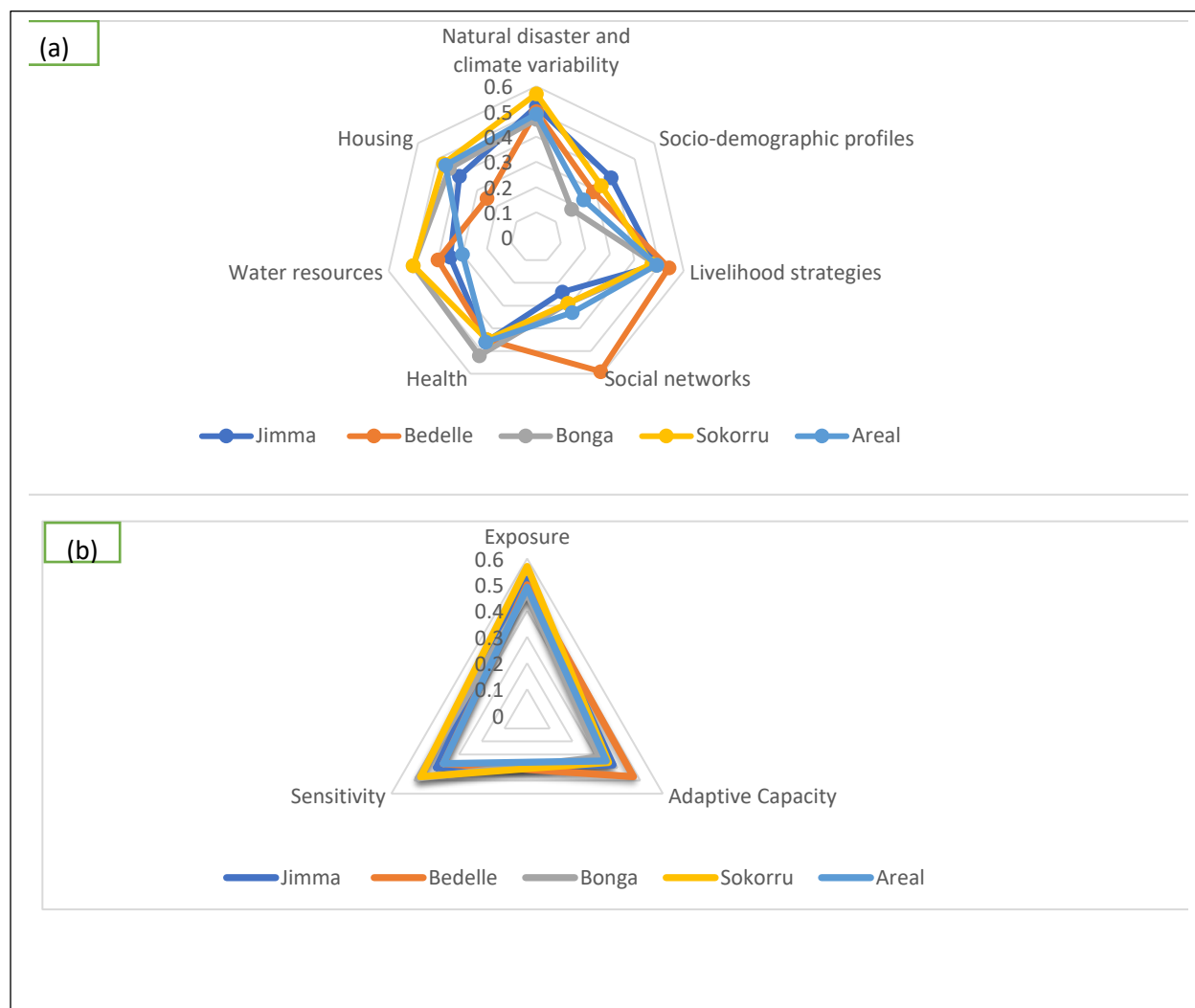
Figure 3. Distribution diagram of vulnerability for (a) the LVI components (b) LVI-IPCC model
