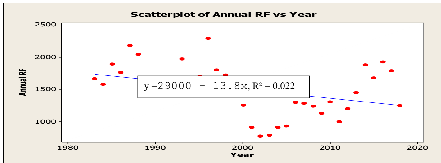
Figure 3. Annual rainfall trend of Begi District area (from 1983-2018).
