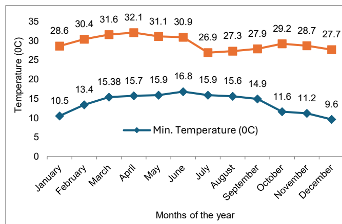
Figure 2. Long-term mean maximum and mean minimum temperatures at Melkassa (1987-2017)
