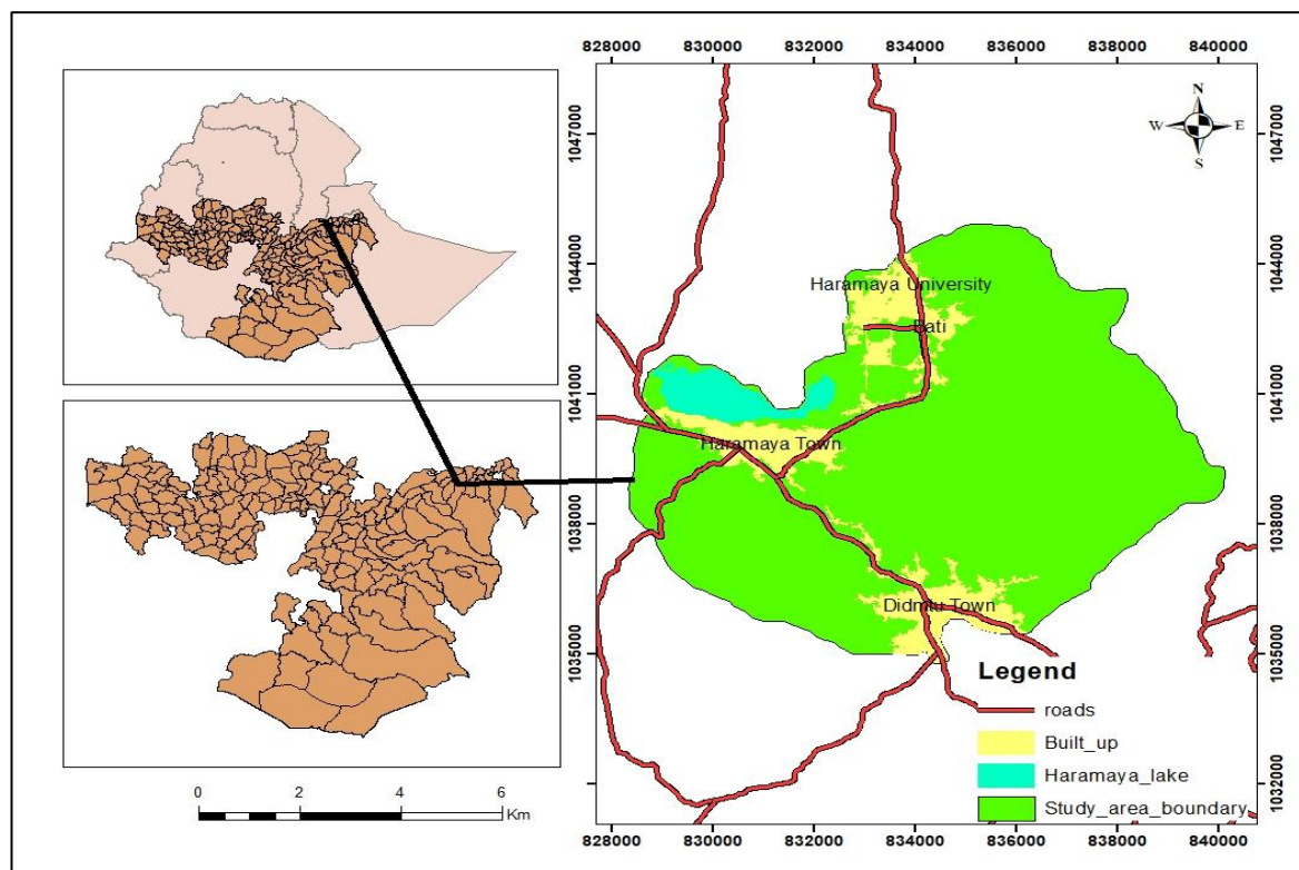
Figure 1. Local map of the study area.
