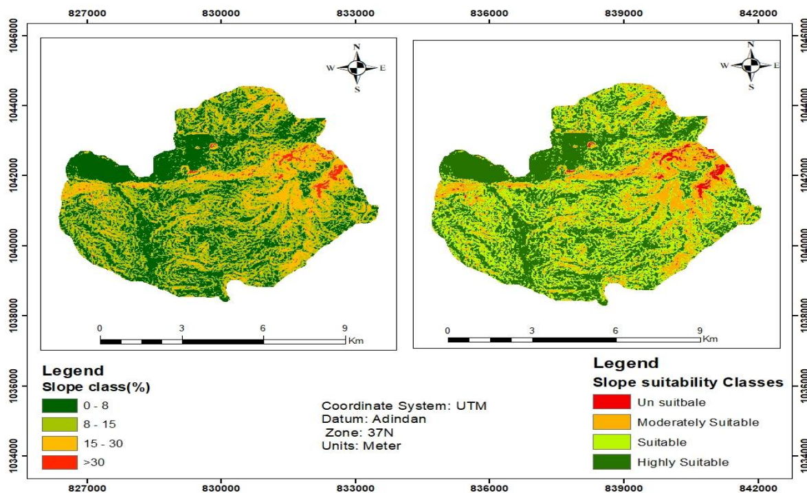
Figure 8. Slope classes and suitability map
