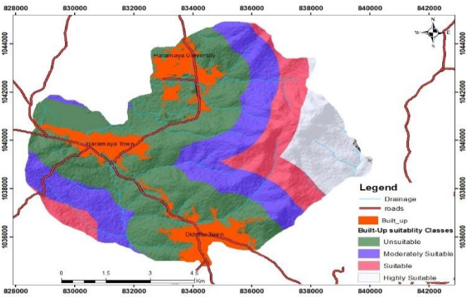
Figure 4. Settlement (built-up) suitability index
