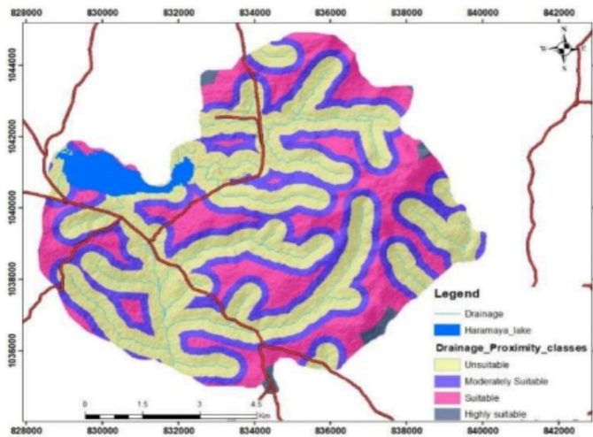
Figure 7. Drainage suitability map
