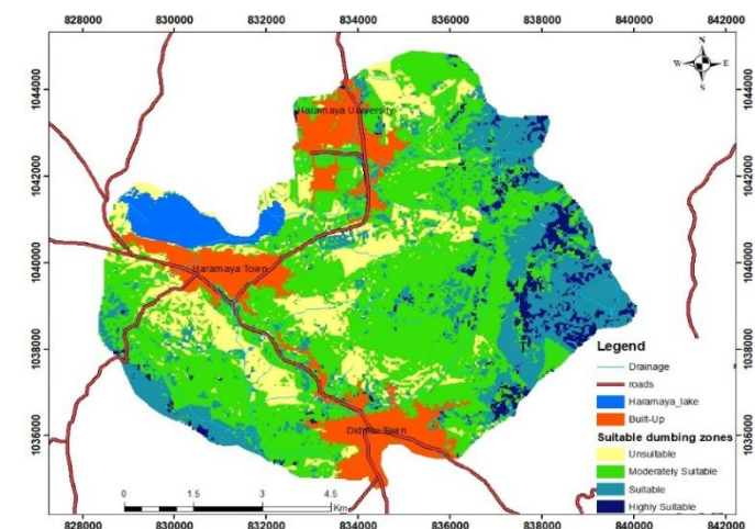
Figure 12. Final suitability map of waste disposal site
