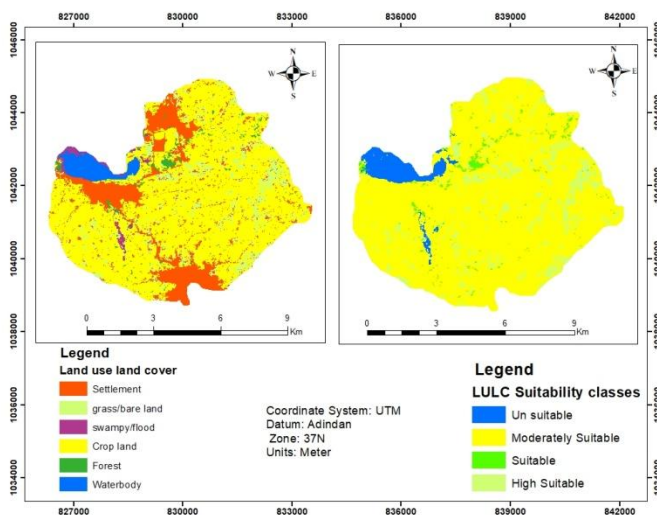
Figure 3. LULC types and suitability index
