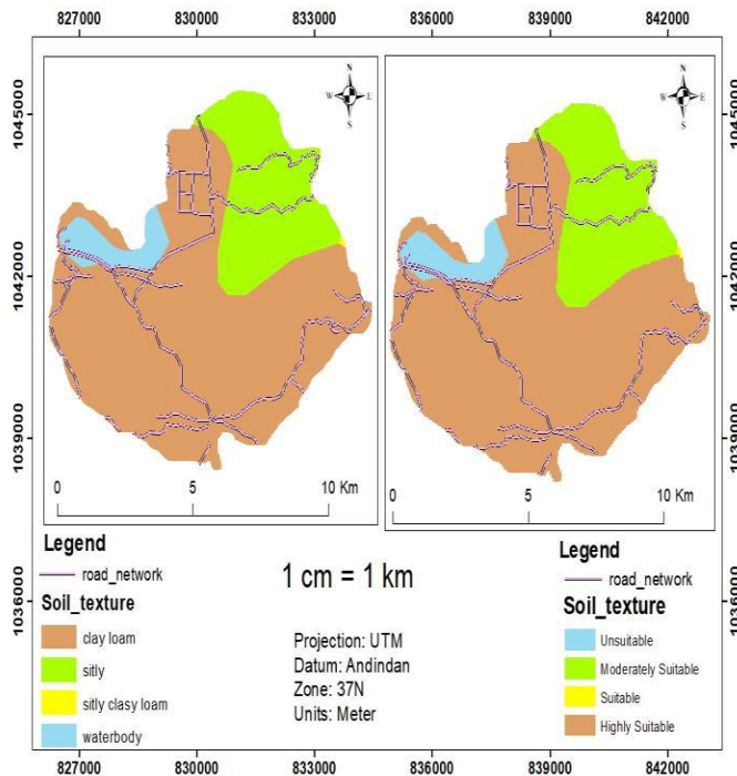
Figure 11. map of soil texture suitability classes
