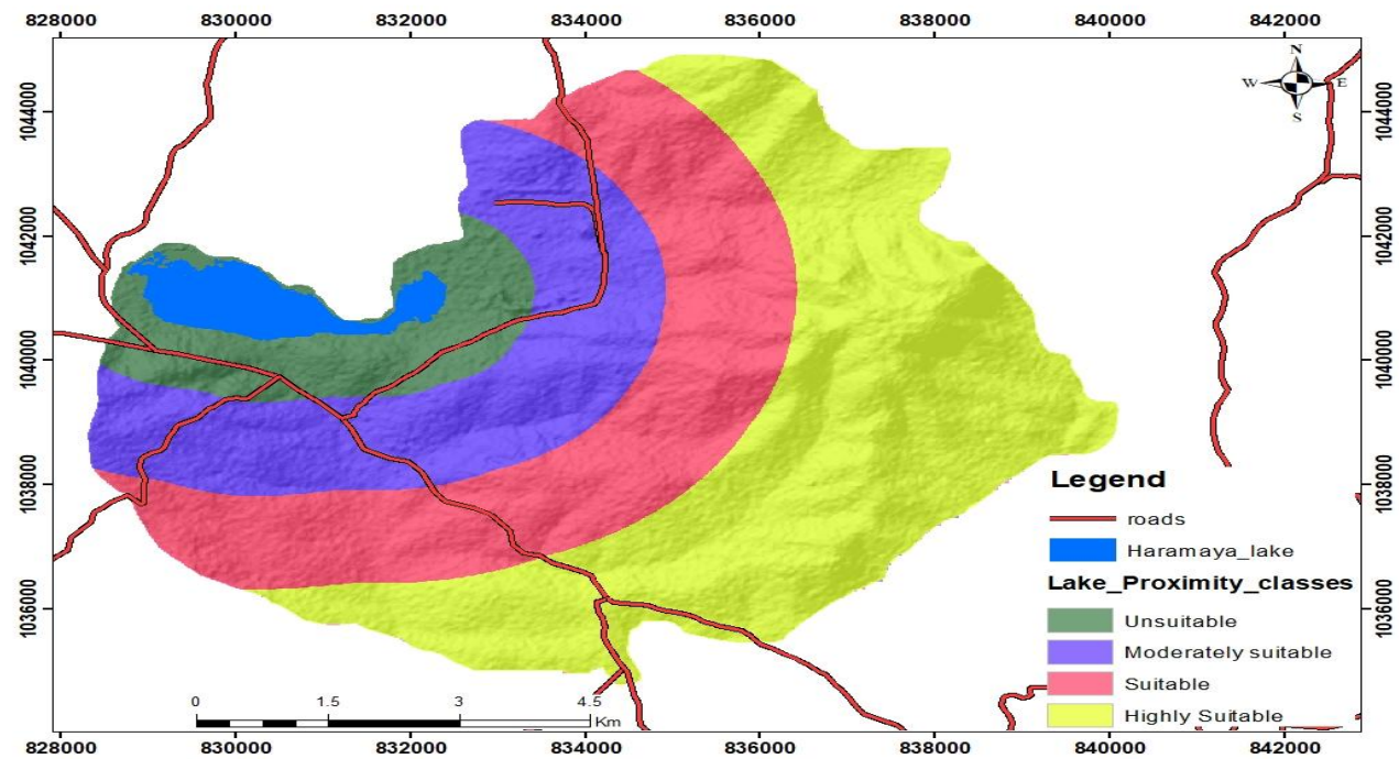
Figure 6. Lake Proximity suitability map
