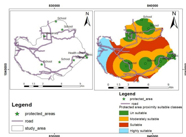
Figure 10. Protected area suitability map
