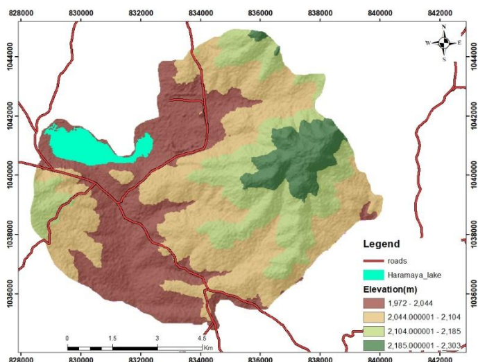
Figure 9. Elevation suitability index
