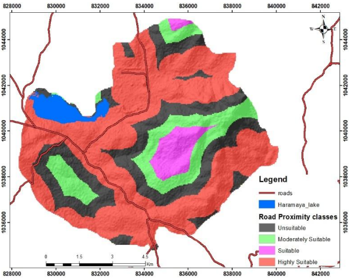
Figure 5. Road network suitability map
