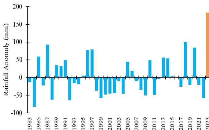
Figure 8. Anomaly histogram of mean MAM season total rainfall from long-year mean value (1983-2022) over 40 years (1983 - 2023) in Ethiopia. The 2023 MAM season anomaly indicated with odd (Orange) color.
