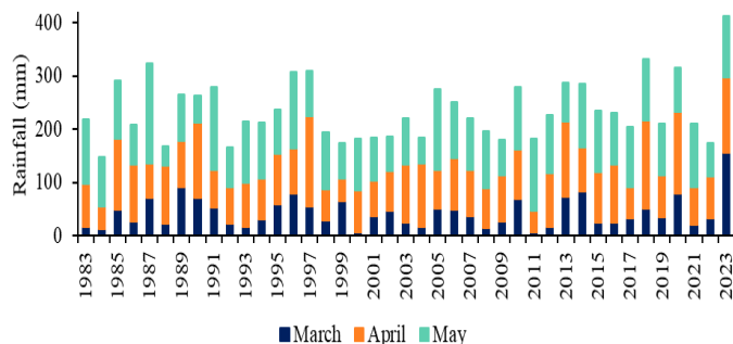
Figure 3. The monthly total rainfall values (in mm) for March, April, and May and the total rainfall for the MAM season for each year from 1983 to 2023 across Ethiopia
