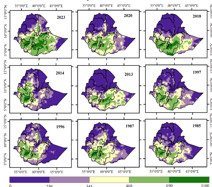
Figure 11. Comparison of the spatial distribution of MAM season total rainfall of 2023 with the selected years having positive and higher anomaly values above the mean MAM season total rainfall across Ethiopia.
