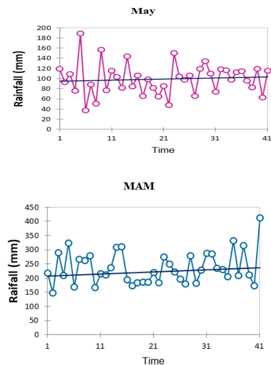
Figure 7. Trends of March, April, May, and MAM from 1983 to 2023 (41 years) in Ethiopia with Sens slope (in mm).
