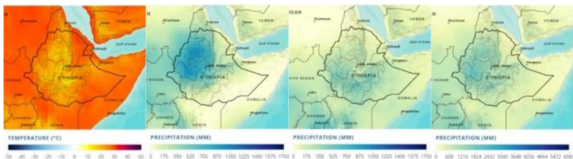
Figure 1. Spatial distribution of mean annual temperature (a), JJAS season rainfall (b), MAM season rainfall (c), and Annual rainfall (d) of Ethiopia (Adopted from World Bank Climate Change Knowledge Portal , 2020)
