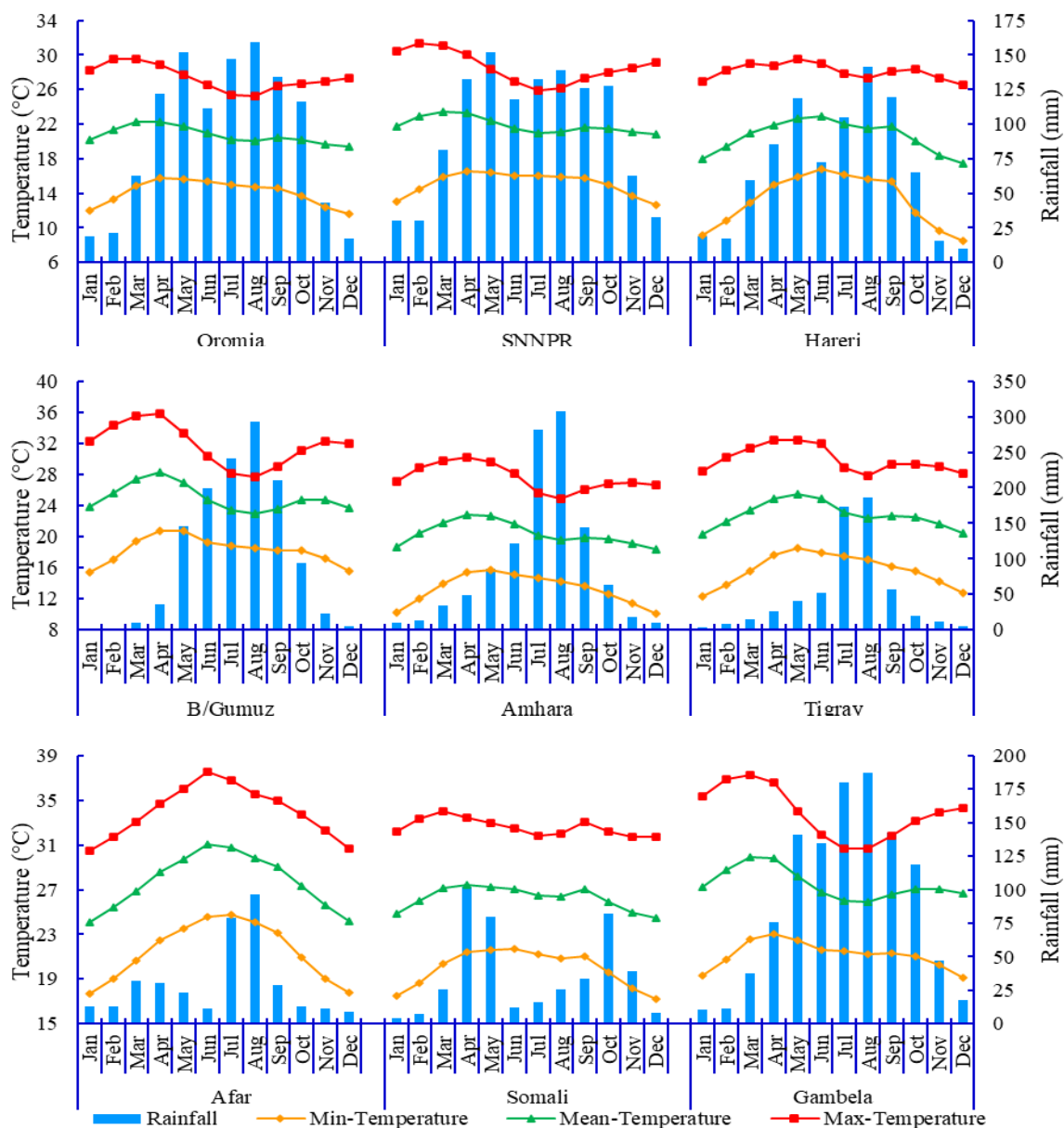
Figure 2. Monthly rainfall, maximum temperature, minimum temperature and mean temperature distribution of the nine regions of Ethiopia (Based on the data obtained from the World Bank Climate Change Knowledge Portal , 2020).
