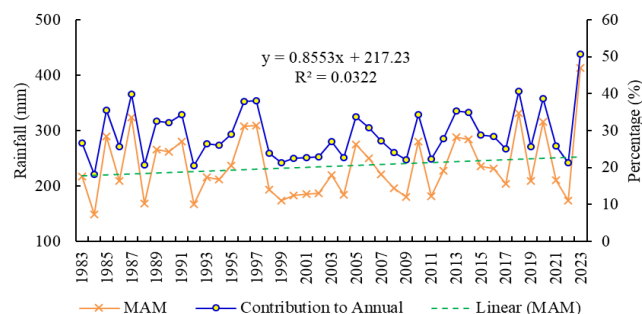
Figure 5. MAM season rainfall amounts and their contribution to annual rainfall total in Ethiopia from 1983 to 2023 (41 years). The linear trend line indicated with a dashed green line shows an increasing trend of MAM season rainfall at the country level.
