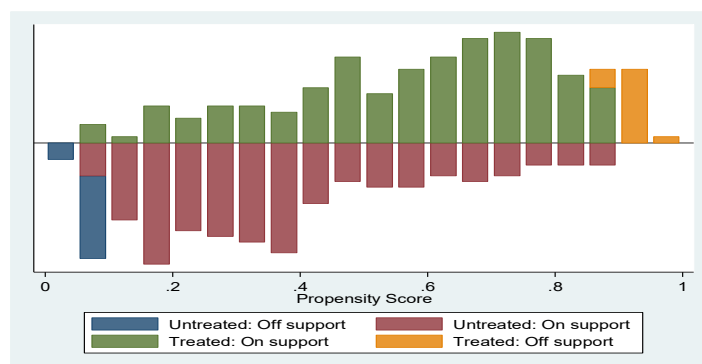
Figure 2. Propensity score
