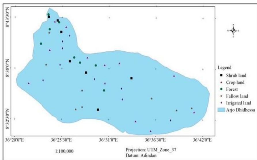
Figure 3. Spatial distribution of the actual soil sampling points at the study site
