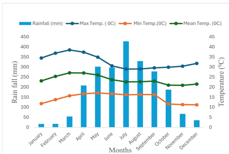
Figure 2. Rainfall and temperature distributions in the study area
