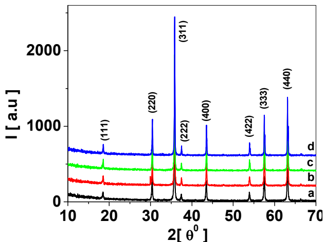
Figure 1: X-ray diffraction patterns of \text{CoFe}_2\text{O}_4 samples annealed at temperatures (a) 300 °C, (b) 500 °C, (c) 700 °C and (d) 900 °C
