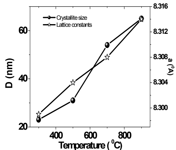
Figure 2: Dependence of crystallite size ( D ) and lattice constants ( a ) on the annealing temperatures of \text{CoFe}_2\text{O}_4 samples
