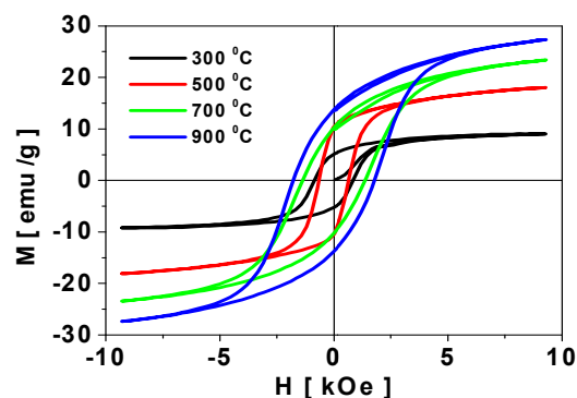
Figure 5: Room temperature magnetization measurements for \text{CoFe}_2\text{O}_4 samples annealed at different temperatures
